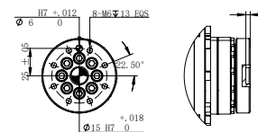
Flange Installation Diagram
