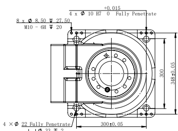
Base Installation Diagram
