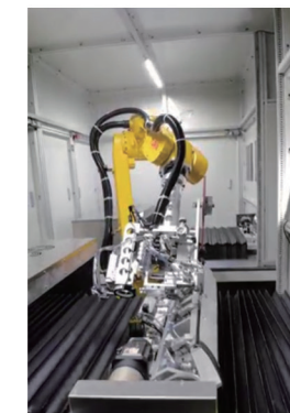
Gluing of washing machine covers
