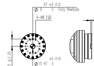
Flange Installation Diagram
